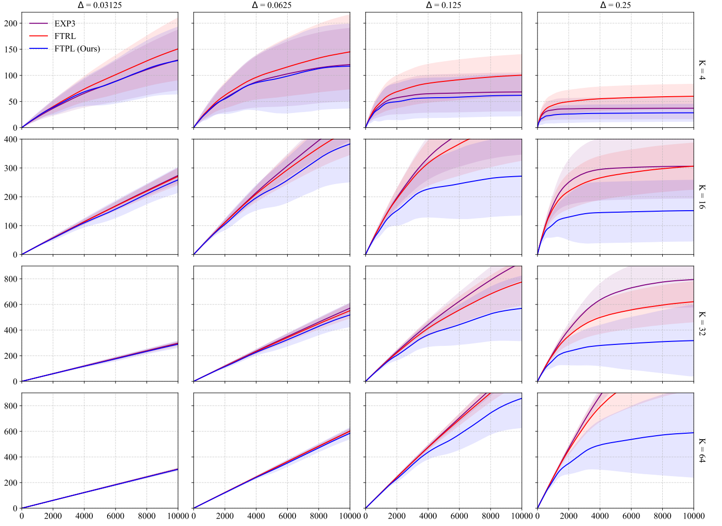
Figure C: Adversarial settings with various choices of the number of arms K \in \{4, 16, 32, 64\} and the suboptimality gap \Delta \in \{0.03125, 0.0625, 0.125, 0.25\} considered in Zimmert & Seldin (2021), 1000 independent runs
