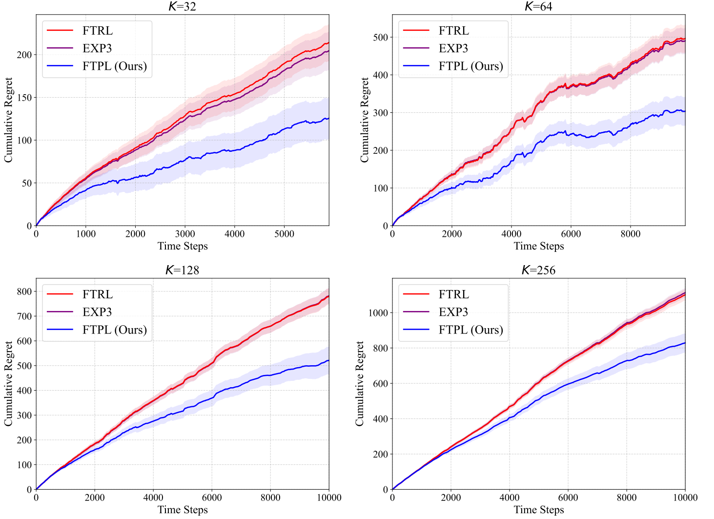
Figure B: Real-world data-based experiments, where we construct a robust offline oracle using the Movie-Lens 100K dataset to simulate online setting. 100 independent runs
